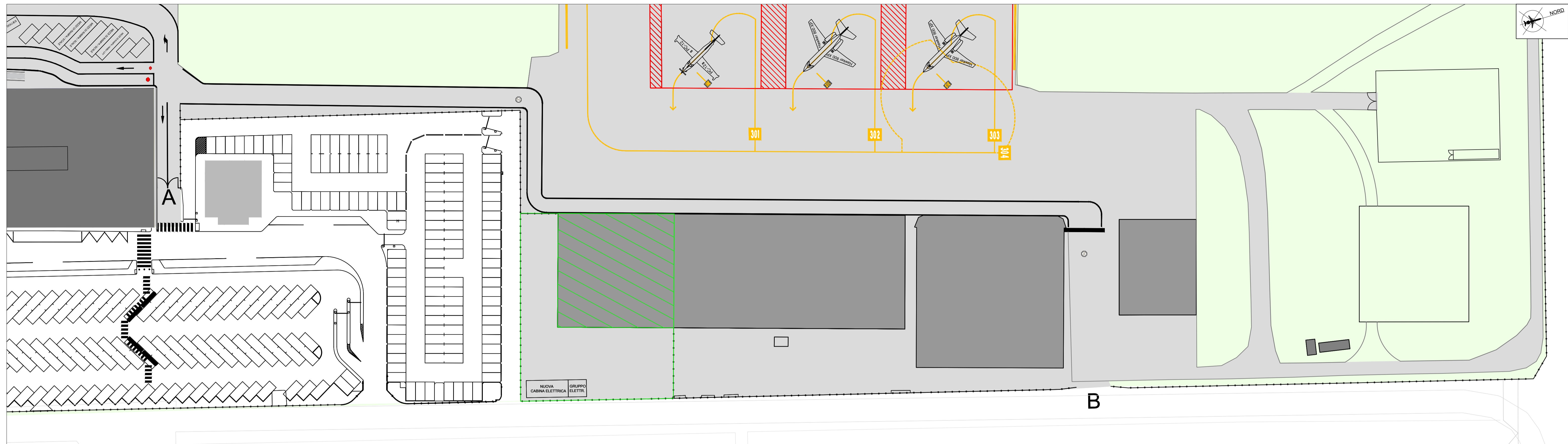
HANGAR - PIANO TERRA, scala 1:100
